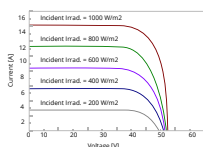
IV CURVE
