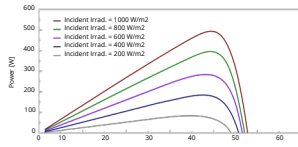
PV CURVE
